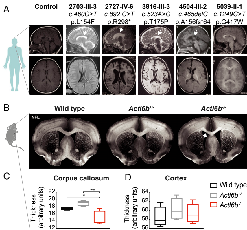
Fig. 3. Loss of ACTL6B causes corpus callosum hypoplasia in humans and mice. (A) Human brain MRI scans of control compared with ACTL6B mutated subjects. (Top row) Midline sagittal. White arrows: corpus callosum hypoplasia. (Bottom row) Axial images at the level of the foramen of Monroe showing paucity of white matter compared with control. (B) Adult mouse coronal brain slices from wild type, Actl6b +/+ , or Actl6b -/- were stained with antibodies to neurofilament light chain (NFL) to visualize callosal axon tracks. Representative images of male wild-type, Actl6b +/+ , and Actl6b -/- brain slices. Actl6b -/- corpus callosum was visibly thinner, indicated with a white arrow. (C) Quantification of relative callosal thickness showing significantly thinner callosum in knockouts. Blinded measurements from n = 2 slices were averaged for each animal and compared for n = 4 mice per genotype. (D) Quantification of relative thickness of the somatosensory cortex in slices used for C showing no significant difference. Significance was assessed by ordinary one-way ANOVA with Tukey's correction for multiple comparisons; F_{(2,9)} = 10.73 for C; F_{(2,9)} = 0.62 for D. Error bars indicate SEM. * P < 0.05 ; ** P < 0.01 ; *** P < 0.001 .
