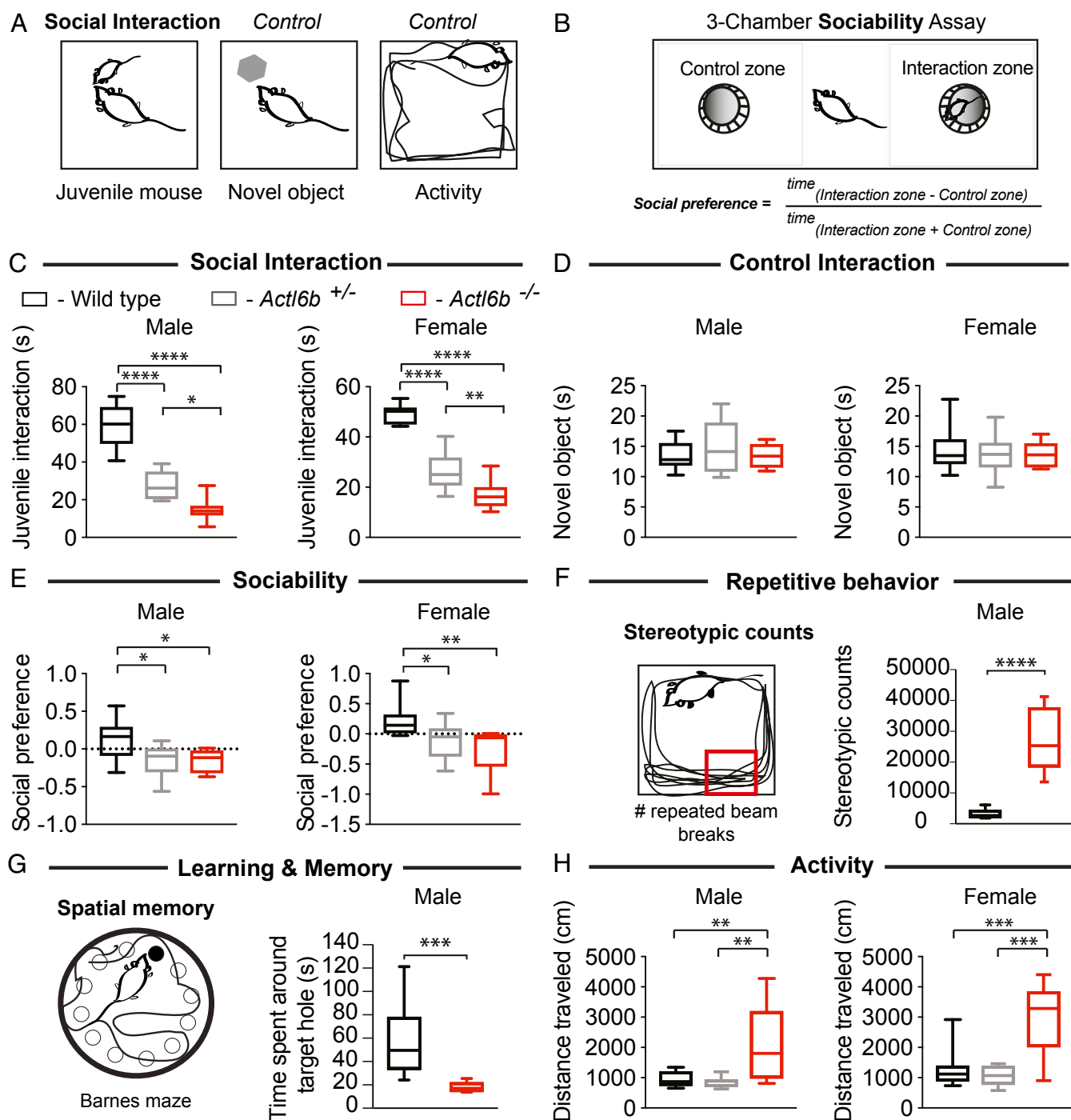
Fig. 4. Actl6b -/- mice exhibit autism-related behaviors. (A) Social interaction and control tests: relative interaction time between the adult test mouse and a juvenile mouse (3–5 wk) or novel object. Open-field test measured activity over 20 min as total distance traveled. (B) Schematic of three-chamber sociability assay: Test mice may enter the zone with a novel object or the zone with a novel juvenile mouse. Social preference scores were calculated from time spent in each zone using the formula shown. (C) Box plots showing male and female littermates of Actl6b +/- × Actl6b +/- crosses with gene dosage-dependent impairment in social interaction with a juvenile mouse but not with (D) a control novel object. (E) Actl6b +/- and Actl6b -/- mice of both sexes showed defects in sociability, which were most severe in female knockouts. (F) Single, repeated photobeam breaks or “stereotypic counts” represented by a small red box in an open field. Male Actl6b -/- mice showed repetitive movements indicated from increased stereotypic counts over 120 min. (G) Diagram of Barnes maze test of spatial memory: an elevated, white, circular open field containing 12 holes, with one “target” escape hole leading to a comfortable cage. Visual cues provided the mouse with a frame of reference for the location of the target hole. Male Actl6b -/- mice spent less time around the target hole, indicating impaired memory as to the location of the target hole. (H) Actl6b -/- mice of both sexes showed increased activity, not observed in Actl6b +/- . Tests shown in C, E, and H were conducted at Stanford University on a cohort of mice highly backcrossed to the C57BL/6 background; mice ( +/+ , +/- , -/- ): n = 9, 12, 7 males, n = 11, 12, 10 females for C; n = 10, 13, 6 males, n = 11, 12, 9 females for D; n = 10, 12, 7 males, n = 11, 12, 9 females for E; n = 10, 13, 6 males, n = 11, 11, 5 females for H. Values for each test in this cohort were as follows: F_{(2,30)}\text{Females} = 79.87 and F_{(2,25)}\text{Males} = 59.49 for C; F_{(2,29)}\text{Females} = 0.29 and F_{(2,26)}\text{Males} = 0.74 for D; F_{(2,29)}\text{Females} = 6.82 and F_{(2,26)}\text{Males} = 4.83 for E; and F_{(2,24)}\text{Females} = 13.44 and F_{(2,26)}\text{Males} = 8.60 for H. Stereotypic counts in F and spatial memory in G were assessed at Fujita Health University on adult male mice that were the F 1 offspring of a cross between Actl6b +/- 129SvEv × Actl6b +/- C57BL/6. Mice ( +/+ , -/- ): n = 22, 21 in F, and n = 22, 14 in G. Significance was calculated for B, E, and H using a one-way analysis of variance (ANOVA) with Tukey’s multiple-comparison post hoc. Significance for F and G was calculated using Student’s t test: t_{41} = 8.68 in F and t_{34} = 3.99 in G. Whiskers indicate 10th and 90th percentiles. * P < 0.05; ** P < 0.01; *** P < 0.001; **** P < 0.0001.
